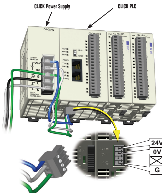
24VDC Output Power Terminals (for CLICK PLC, I/O or field device, etc.)
