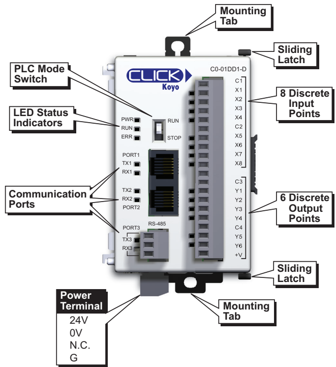
Standard PLCs
