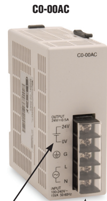
24VDC Output Power Terminals (for CLICK PLC, I/O or field device, etc.)
