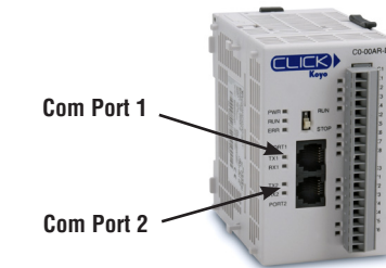
Basic PLC
